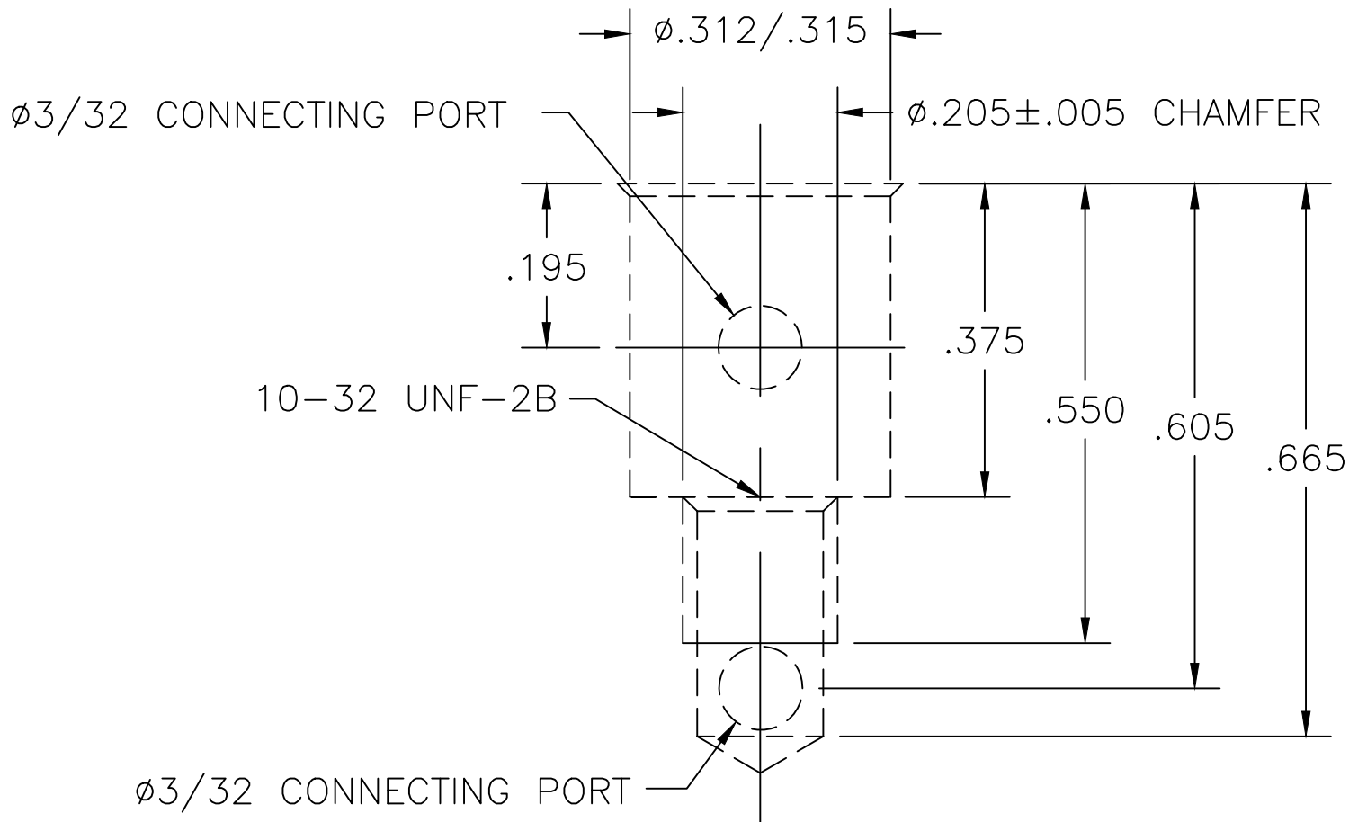
SUGGESTED PORT DIMENSIONS
