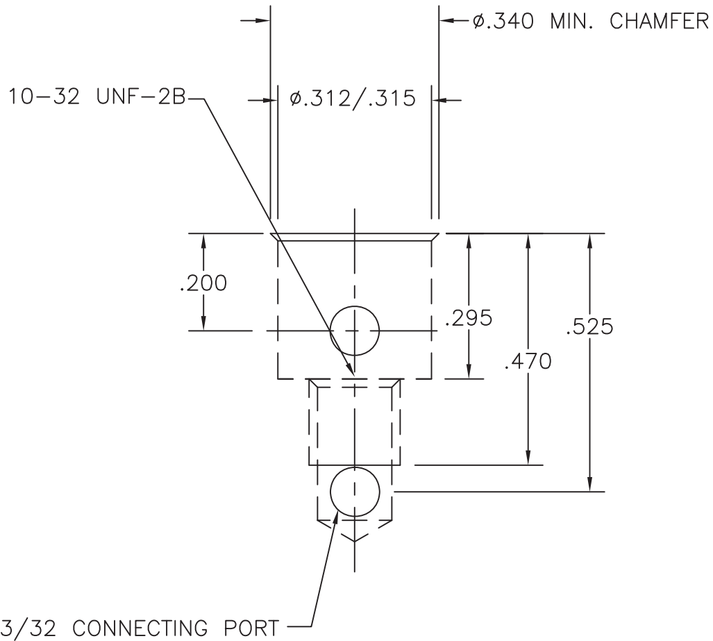
SUGGESTED PORT DIMENSIONS
